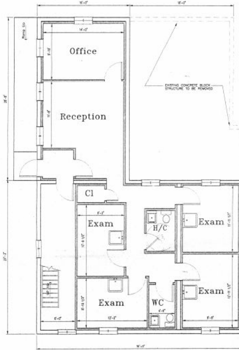
2 Second Floor Plan A1 Scale: 1/4"=1'-0"
